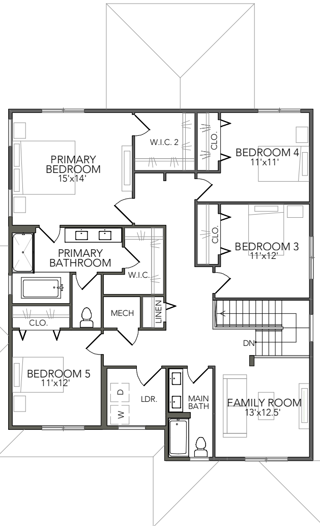
UPPER FLOOR
