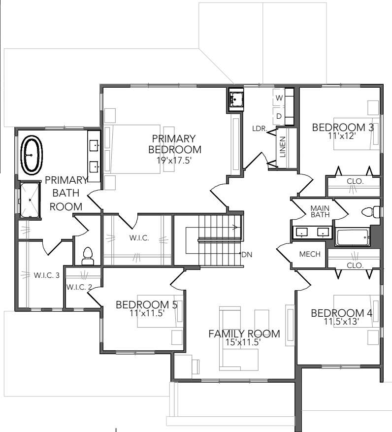
UPPER FLOOR
