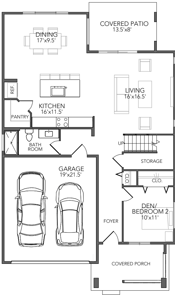
MAIN FLOOR
