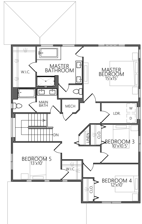
UPPER FLOOR
