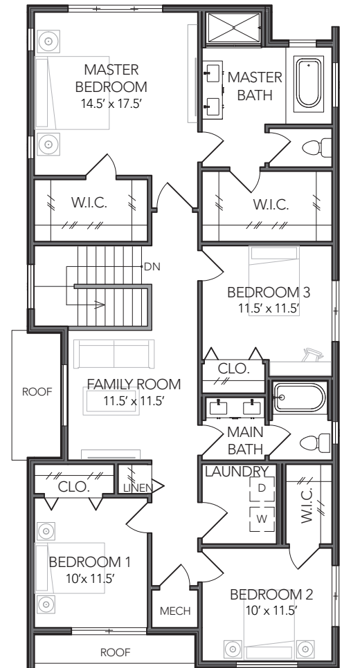
UPPER FLOOR
